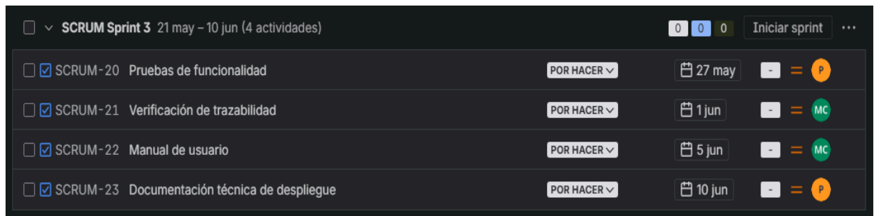
Fig. 2.2.4 Scrum 3
